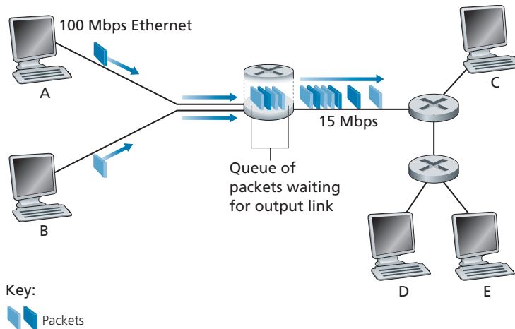
Figure 1.12 ♦ Packet switching
